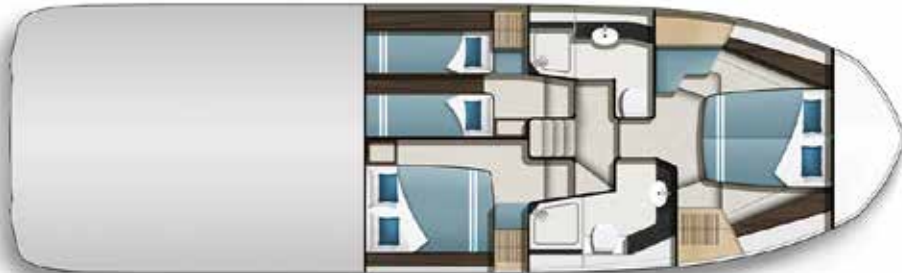
3-CABIN - CONVENTIONAL
